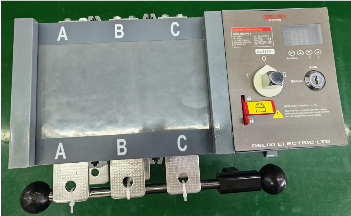
Outer consturction of CDQ6i-800N/3PBD
