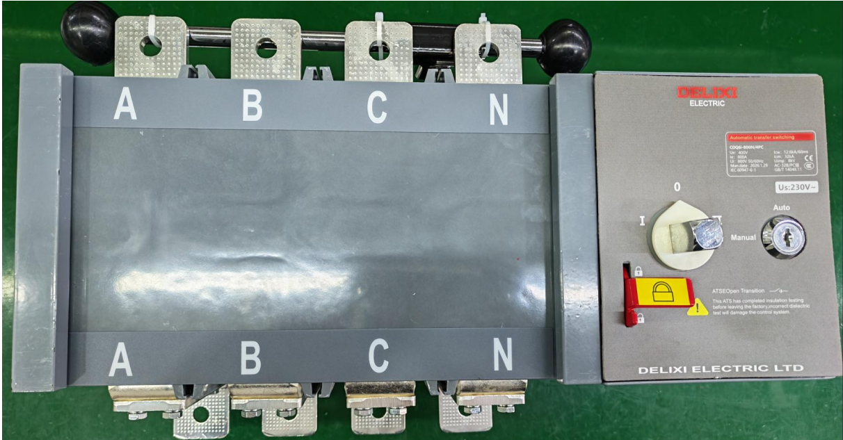
Outer consturction of CDQ6i-800N/4PC
