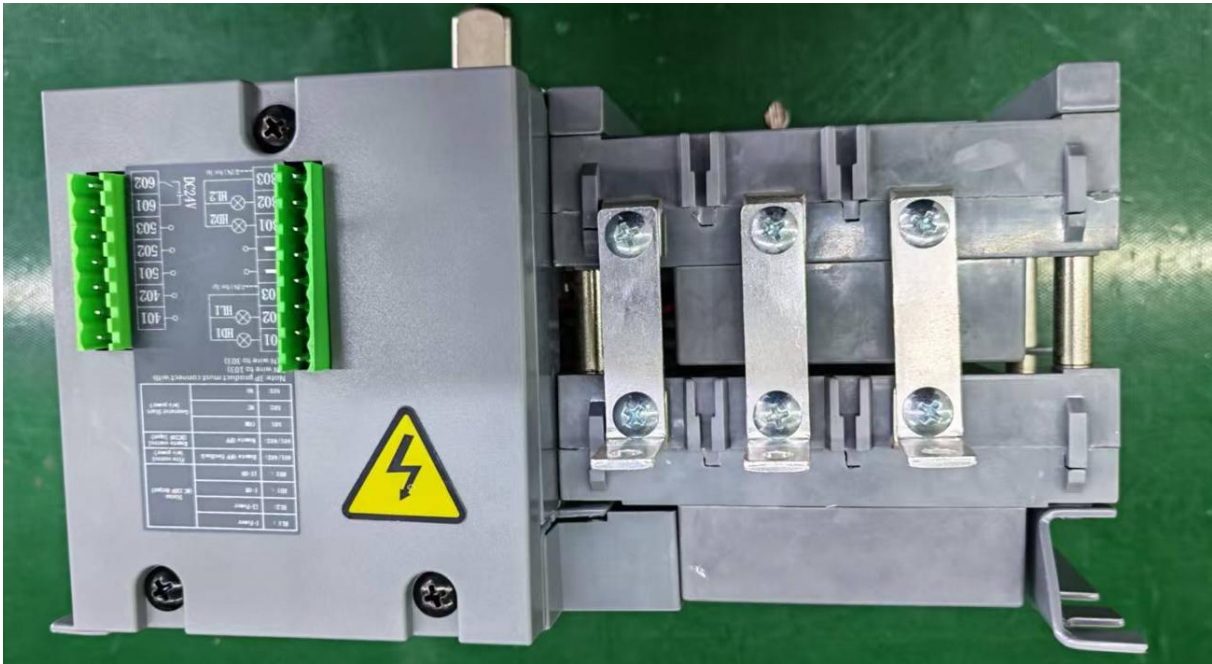
Outer construction of CDQ6i-100H/4P
