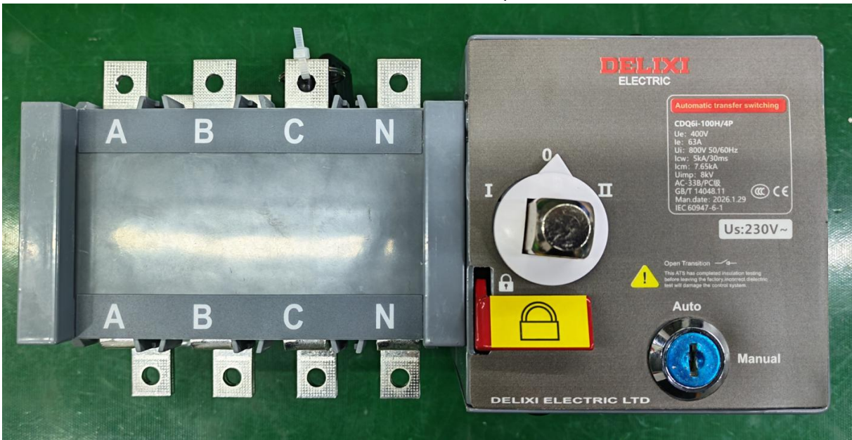
Outer construction of CDQ6i-100H/4P
