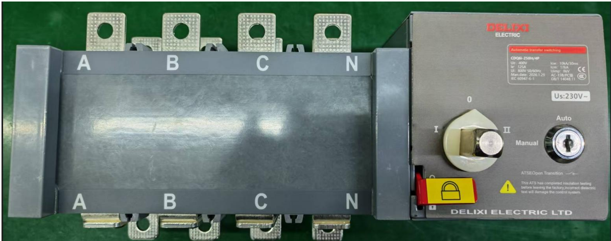
Outer construction of CDQ6i-250H/4P
