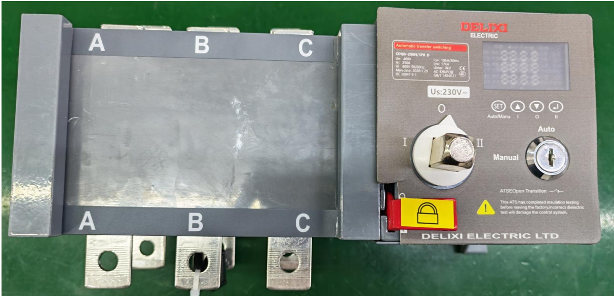
Outer construction of CDQ6i-250N/3PBD
