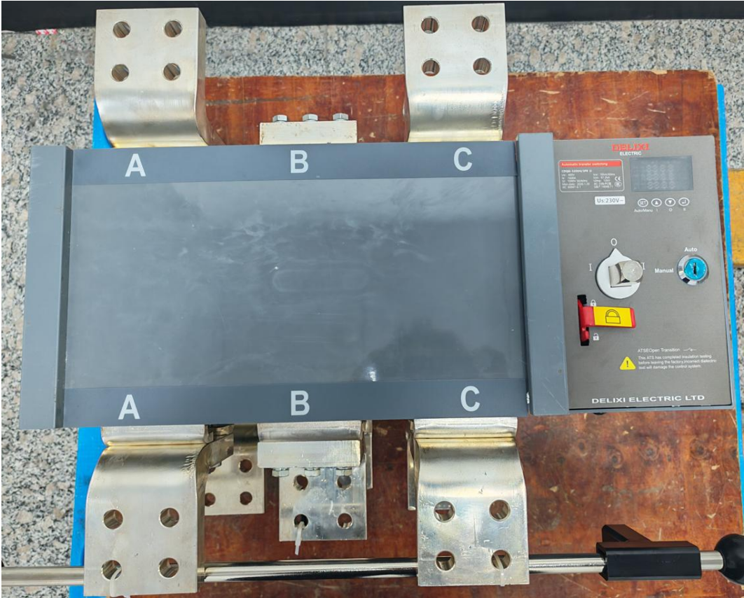
Outer construction of CDQ6i-3200H/3PBD
