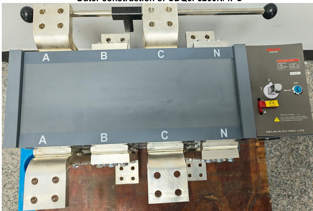
Outer construction of CDQ6i-3200N/4PC
